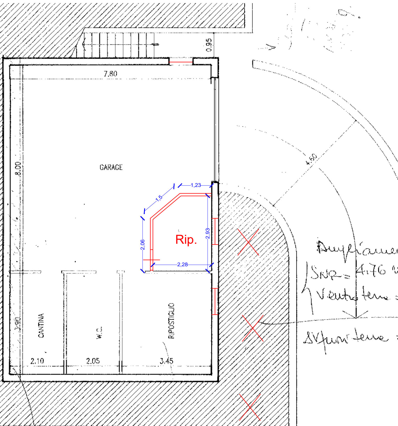
PIANO INTERRATO
